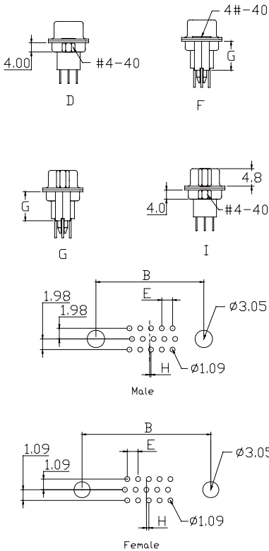
Recommended PCB Layout (PCB TOLERANCE±0.05)
